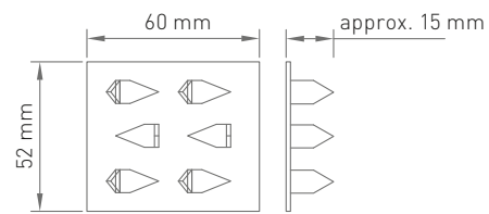
Wall claw for 40/20 mm strong wall absorber, claw height 15 mm
