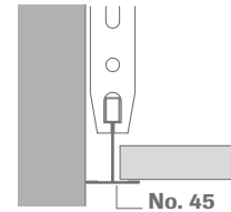
Fixing to the soffit (sliding connection)
