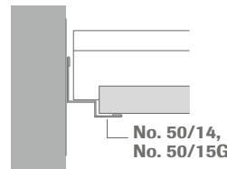
Contura ceilings S 3a and system S 15a cliq
