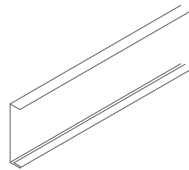
C profile no. 36 height 50 mm
